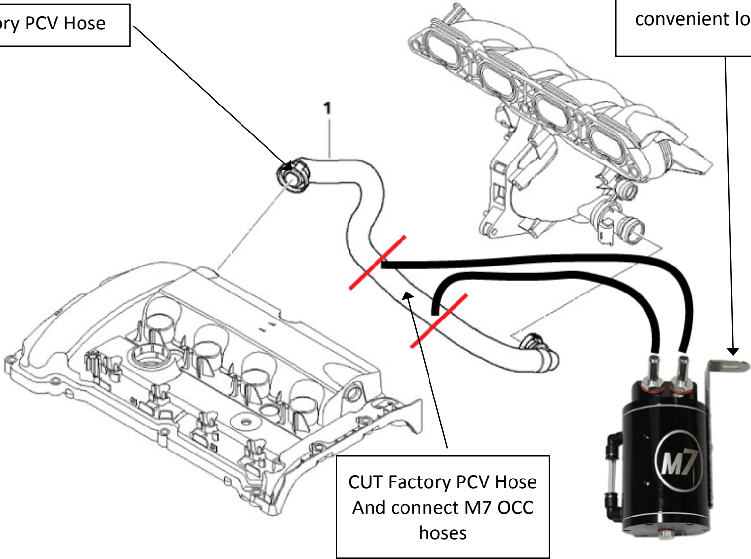
Figure 1: N12B Non-Turbo Engine Oil Catch Can Installation Schematic
